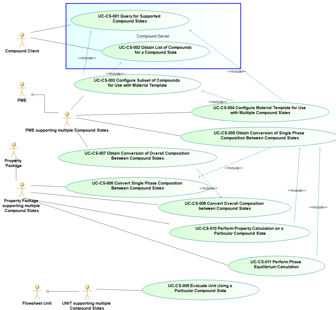
Figure 6-3 Use Case map for Compound Slates
