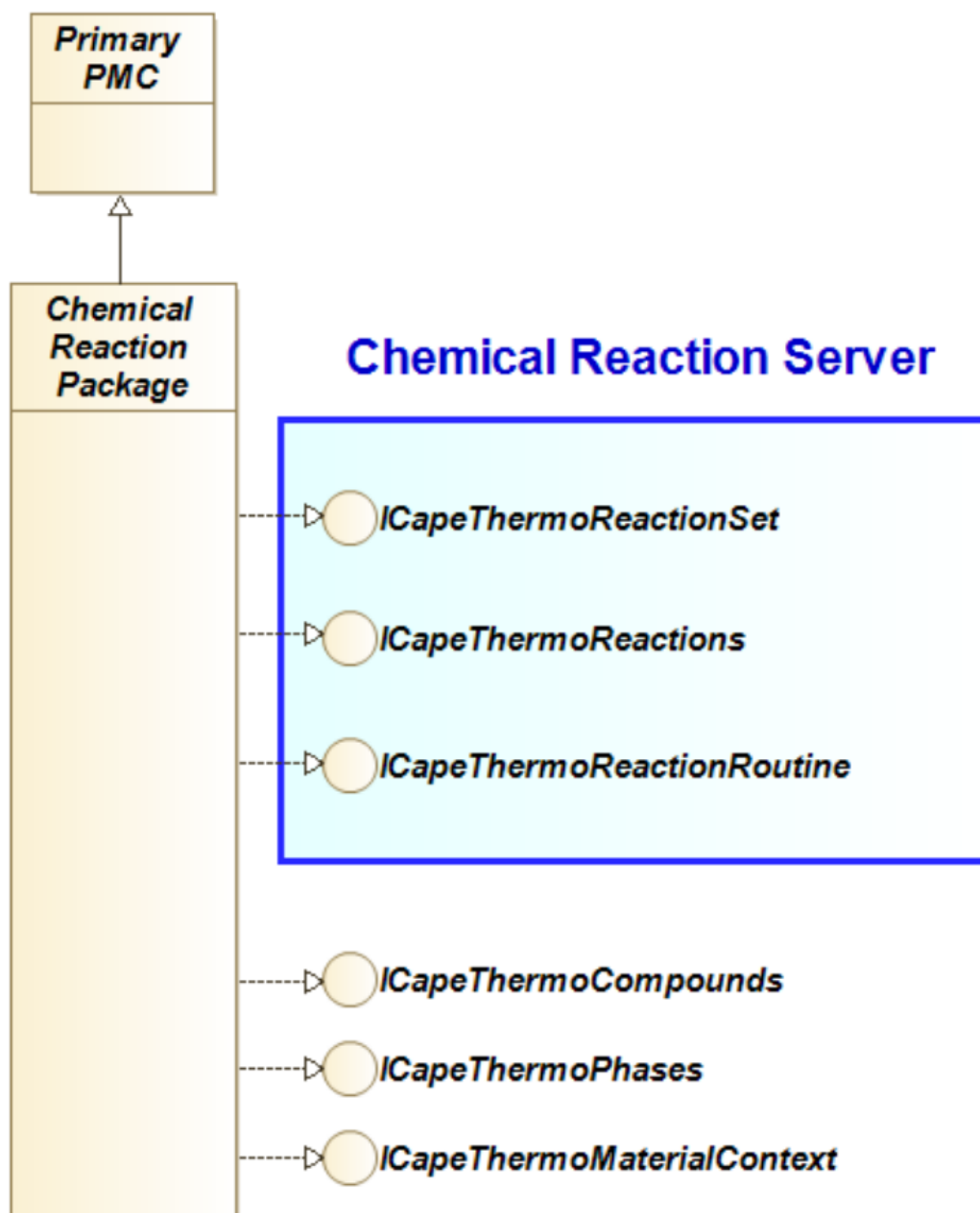
Figure 4-3 Chemical Reaction Package
