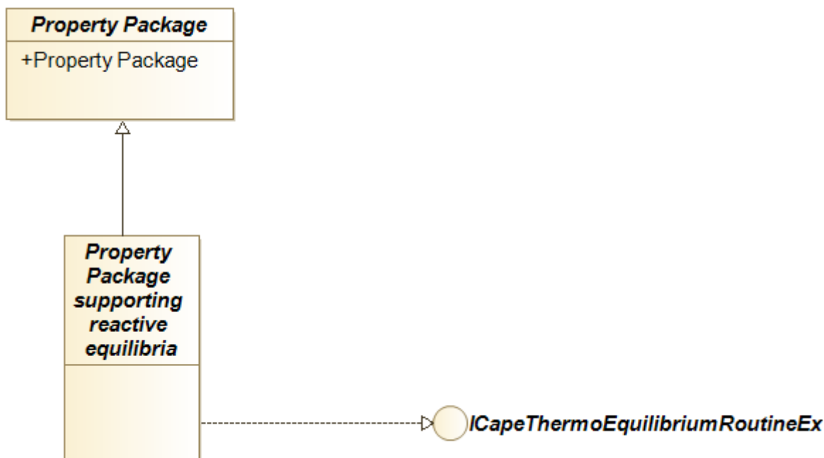
Figure 5-2 Property Package supporting reactive phase equilibria
