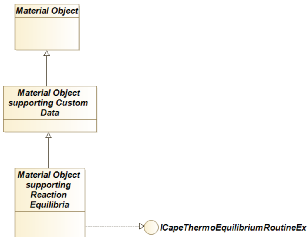
Figure 5-1 Material Object supporting reactive phase equilibria
