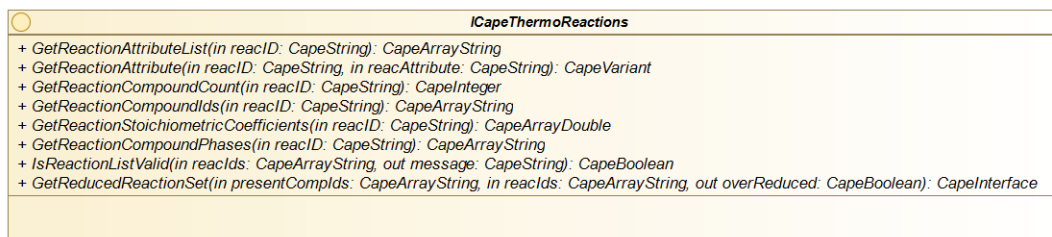
Figure 4-10 Interface diagram for ICapeThermoReactions
